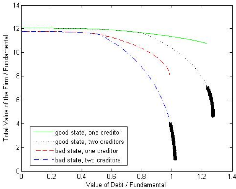
Figure 2 The figure plots the expected total firm value against the expected value of the debt. The solid (dashed) line is the firm value with a single creditor when the fundamental \theta = G ( \theta = B ). The dotted (dash-dotted) line is the firm value with two creditors when the fundamental \theta = G ( \theta = B ). The thick solid black segments can be supported only by two creditors. Although the firm values are comparatively much lower along the thick lines, the firm cannot even reach that portion with just one creditor. When the value of debt is very low the choice between one and two creditors is irrelevant. As the fundamental worsens, the two groups of lines diverge and, when both are feasible, the single creditor structure always delivers a higher firm value.
