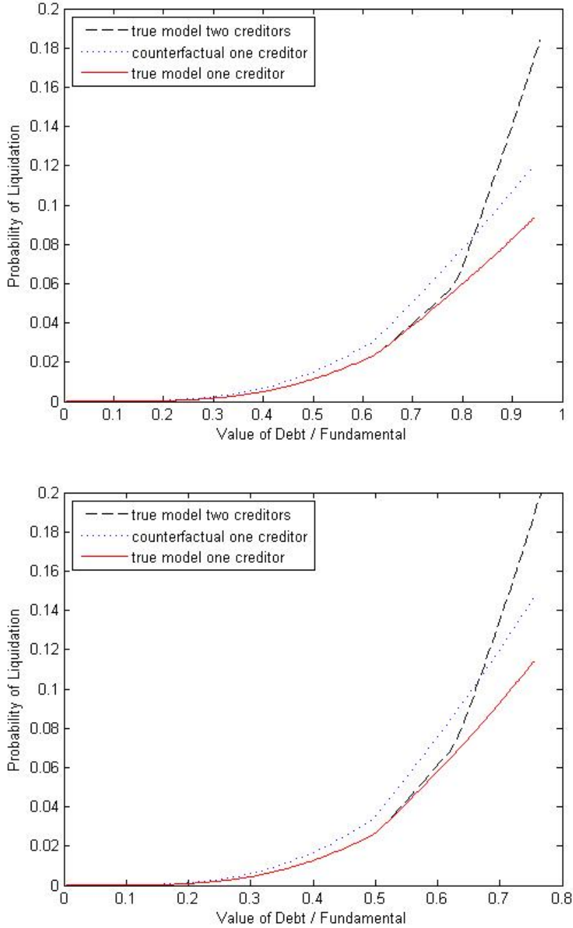
Figure 4 The figure plots the expected probability of liquidation L_1^{\theta,\infty}(F,Y) against the expected value of the debt conditional on the current state \theta = G (top panel) and \theta = B (bottom panel). The solid (dashed) line is the liquidation probability with a single creditor (two creditors) in the full model. The dotted line is for the counterfactual model in which the number
