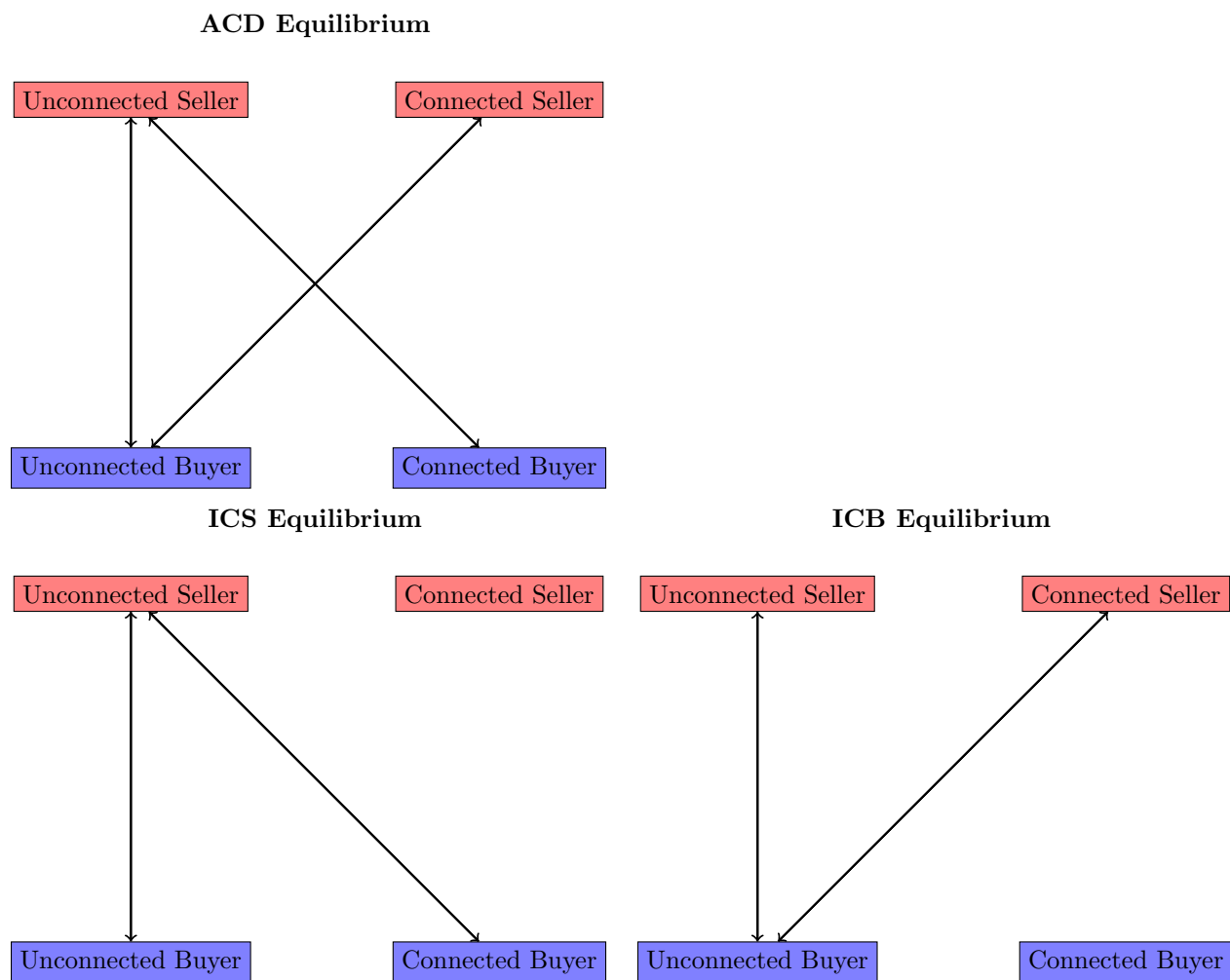
Figure 3: Equilibrium configurations. An arrow going from one type of trader to another indicates that the former makes offers to the latter in equilibrium.
