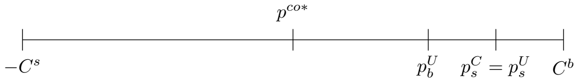
Figure 5: Equilibrium Prices. This figure shows the position of equilibrium prices in the peripheral market relative to the equilibrium core market price in each possible equilibrium regime when \alpha^{pe} > 0.5 and \alpha^{pe} < 0.5 ;
