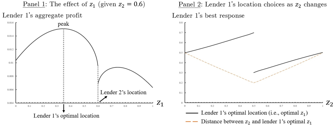
Figure C.3: Lender 1's Optimal Location Choice ( q > 0 ). Panel 1 plots how lender 1's aggregate profit changes as its location z_1 varies. Panel 2 plots lender 1's best response as lender 2's location z_2 varies: The solid curve plots lender 1's optimal location (i.e., optimal z_1 ), while the dashed curve plots the distance between z_2 and lender 1's optimal z_1 . The parameter values are: R = 2.4 , B = 0.9 , b = 0.4 , p = 0.5 , q = 0.6 , c = 1 , and f = 1 in both panels; z_2 = 0.6 in Panel 1.
